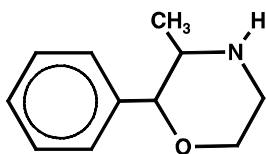
Phenmetracin
